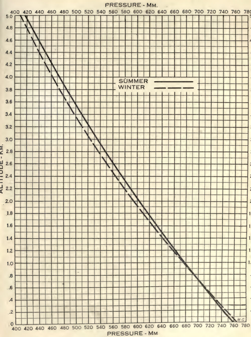
FIGURE 37. Mean summer and winter free air pressures, mm., above Mount Weather, Va. (Extended to sea level.)
